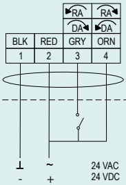
Open/Close, Single Wire Control
