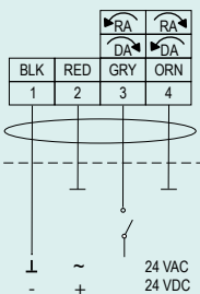
ON/OFF Control, Two Wire
